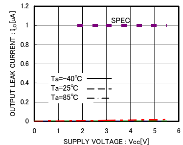
Fig.8 Output leak current I_{II} (SDA)
