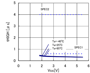
Fig.17 Data clock "H" time t_{HIGH}
