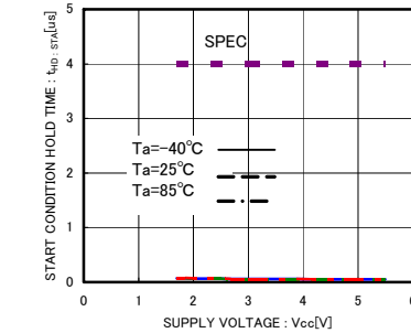
Fig.16 Start Condition Hold Time t HD:STA
