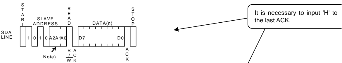
Fig.45 Current read cycle
